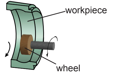
Profile Grinding
