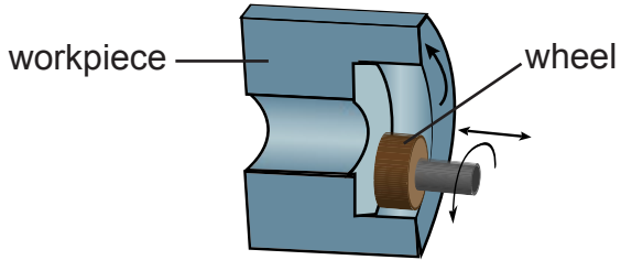
Traverse Grinding
